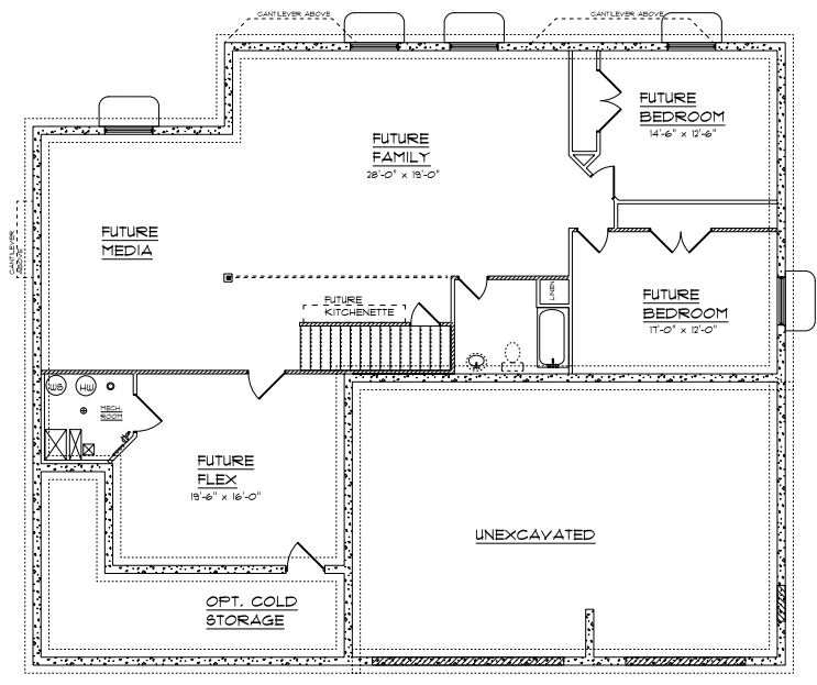
FOUNDATION PLAN
