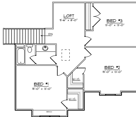
UPPER LEVEL PLAN
